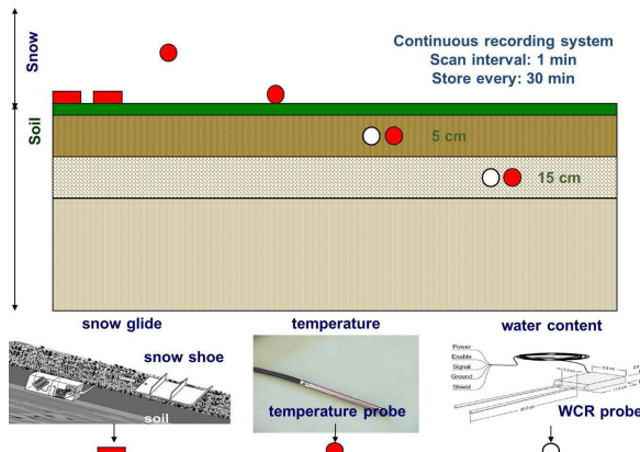
Fig 3: instruments placed in each plot (NB: water content probes in B were put only from 2011).
