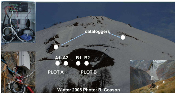
Fig. 2: monitoring site in the glide crack area (A1-A2 and B1-B2 points indicate the glide shoes).
