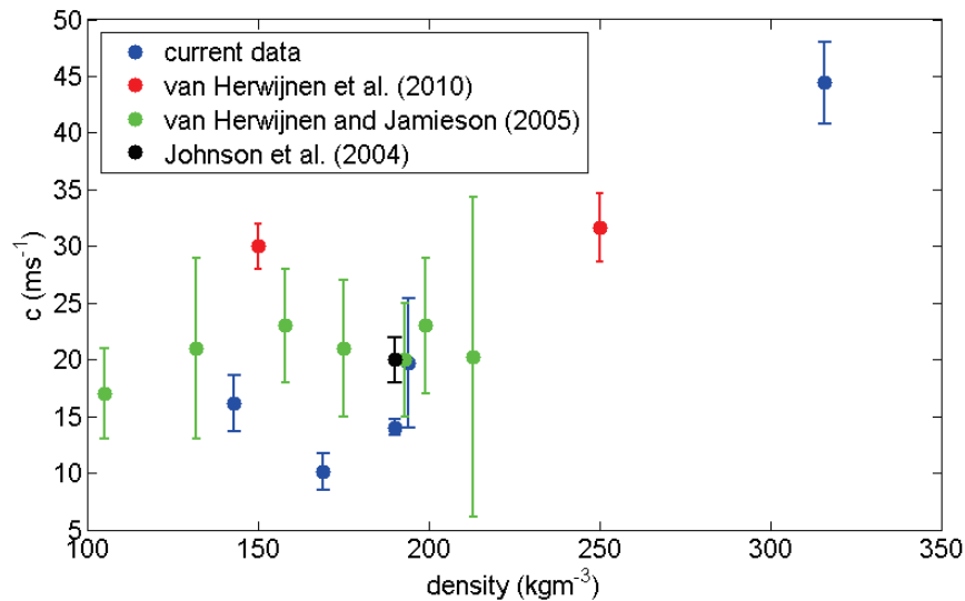
Figure 4: Fracture speed with slab density. Data from this study are shown, as well as data from van Herwijnen et al. [2010], van Herwijnen and Jamieson [2005], and Johnson et al. [2004].
