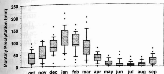
Figure 3: Monthly precipitation at Chacaltaya, Bolivia (5,220 m), 1967–1997. Whisker plot boxes illustrate the median (line) and enclose the 25 th and 75 th percentiles. Error bars enclose the 10 th and 90 th percentiles, with extremes indicated by circles. Annual precipitation averaged 560 mm during this period.
