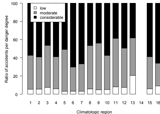
Figure 10: Ratio of recreational avalanche accidents for danger level 'low', 'moderate' and 'considerable' in 16 climatologic regions.
