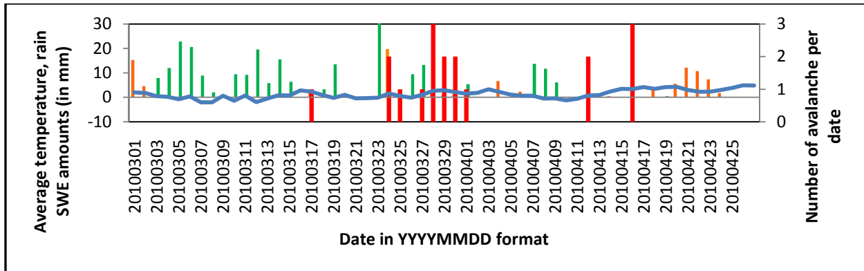
Figure 9: Twenty-four hour average temperatures (in blue), avalanche occurrences (in red), mm of rain, rain (in orange) and mm of SWE (in green) during March and April 2010. Temperature, rain and SWE are in the left axis and avalanche occurrences are in the right axis.
