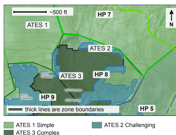
Figure 1: Motorized zone units over the operator's ATES layer, part of Hahns Peak, Colorado; labels, legend and north arrow set in type over an unaltered catalogue view. Solid Colored Lines are zone boundaries. Example: at roughly 1500ft wide HP 8 alone spans Classes 1–3: would be a complex zone (Section 6.4).
