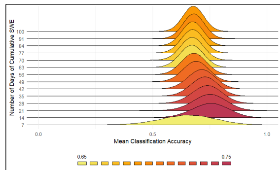
Figure 3: Ridge plot histograms of model performance for each time frame. Darker colors with a peak further to the right of the chart indicate higher percent accuracy
