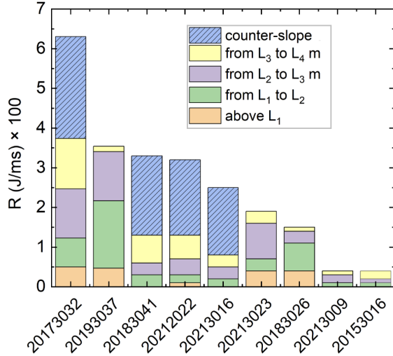
Figure 5: The rate of change in cumulative intensity per unit time between consecutive locations L_{i-1} and L_i , R(t_i) , is plotted for the most energetic avalanches in our dataset. Each color represents a specific section of the path. Avalanches that reach the counterslope with very high energy generate abrupt rapid pressure disturbances, which are indicated in the graph by a pastel blue hatched area.
