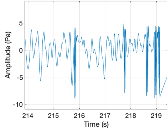
Figure 6: Detail of the infrasound signal generated by the avalanche #20213022 on the counter slope showing sudden and pronounced fluctuations, indicating abrupt rapid pressure disturbances. These disturbances typically have a brief duration, representing single, sharp pulses of energy.
