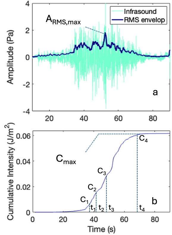
Figure 2: (a) Infrasound signal of avalanche #20150020 with its RMS envelope. (b) Cumulative intensity calculated from the RMS envelope.
