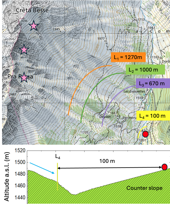
Figure 1: Overview map of the VdIS test site (upper panel). The pink stars highlight the positions of the main release areas, while the red dot marks the location of the infrasound sensor and the GEODAR. Colored lines represent the reference locations. The lower panel shows a sketch of the topography at the bottom of the slope, near the infrasound sensor. A counterslope in this area abruptly halts avalanches, potentially causing the release of high-energy peaks in the infrasound signal. The blue arrow indicates the direction of the incoming avalanche.
