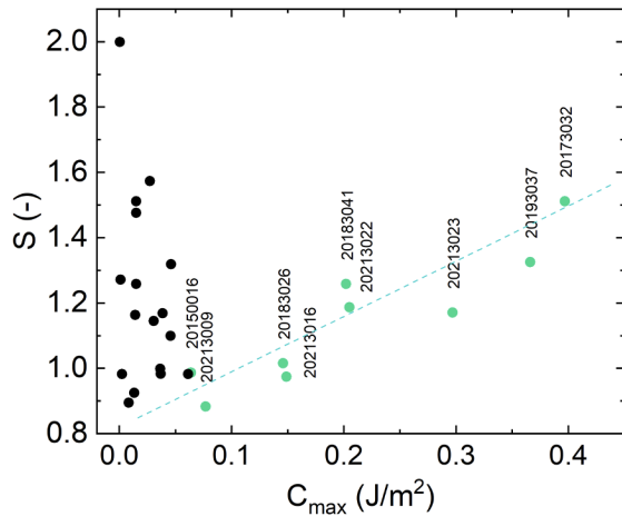
Figure 7: The snow parameter, S , is plotted against the maximum cumulative intensity, C_{max} , for all analyzed avalanches. Green dots highlight the avalanches analysed in Fig. 5. For these avalanches, the maximum cumulative intensity, representing a proxy for the energy of the material in suspension, correlates with snow height and new snow accumulation along the path. The green dashed line serves as a visual guide.
