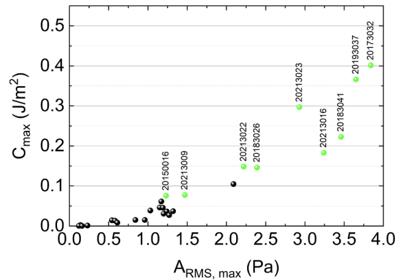
Figure 4: The maximum infrasound RMS amplitude, A_{RMS,max} , is plotted against the maximum cumulative intensity, C_{max} , for all analyzed avalanches. This representation shows that the infrasound signals encompass a wide range of avalanches, characterized by varying degrees of development and energetic content in the airborne layers. Avalanches identified by a reference number and a green dot will be further analyzed in this study.
