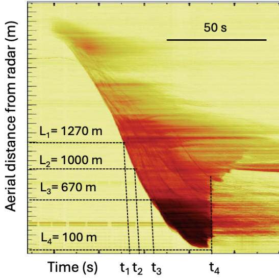
Figure 3: GEODAR radar MTI plot of avalanche #20150020. The reference locations L_1 to L_4 are indicated. Infrasound arrival times t_1 to t_4 have been corrected for acoustic propagation.
