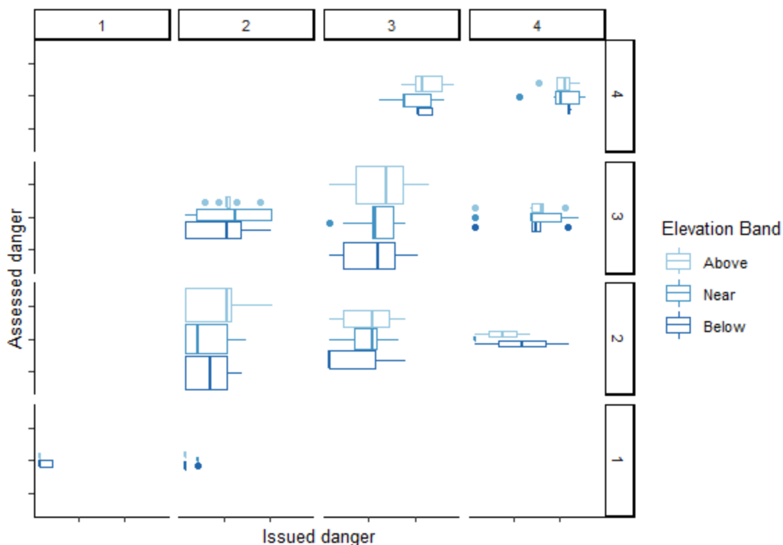
Figure 3. Box plots of log(AAI) by elevation band, presented similarly to the contingency tables. Columns are forecast danger ratings, while rows are assessed dangers. The center diagonal indicates correct forecasts based on assessments, about 84% of total assessments. AAI is exponential, so the log transform makes differences at lower values more visually apparent.
