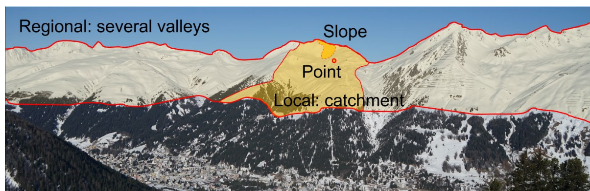
Figure 1: The scales we consider are point, slope, local and regional. The point scale is where we perform stability tests. The slope scale is the starting zone of an avalanche where we assess avalanche release probability (or triggering probability; also called slope stability). The local scale is the basin or catchment we travel in a day and make observations and the regional scale includes several valleys and many basins and is the scale the avalanche forecast is covering, for which the avalanche danger is described in terms of snow stability, its frequency distribution and avalanche size.
