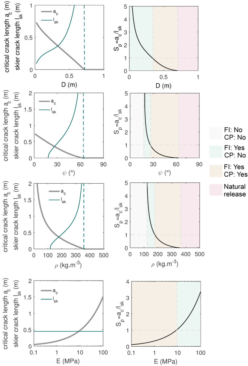
Fig. 4: Sensitivity analysis with independent snowpack properties, i.e. only one parameter was varied while the other properties were kept constant. D=0.4 m, \psi = 30^\circ , \rho=200 kg m -3 , \tau_p = 700 Pa, R=780 N. FI: Failure initiation; CP: Crack propagation.
