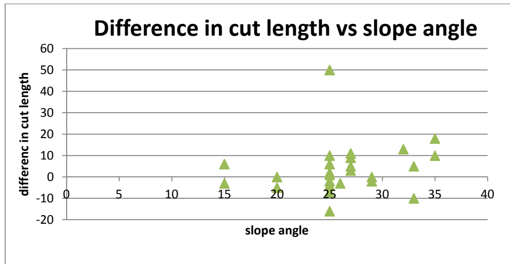
Fig. 3: The difference between the CPST and PST cut lengths and slope angles. Note the divergence in cut lengths once the slope angle gets steeper than thirty degrees.
