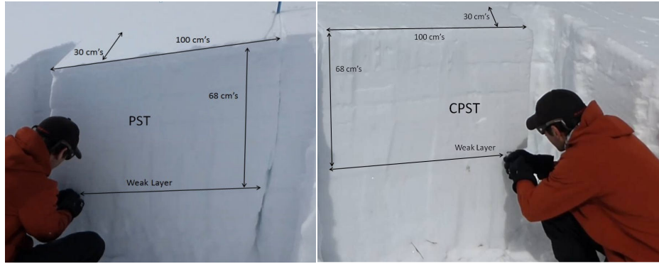
Fig. 1: The photo on the left is a PST in process. The photo on the right is a CPST in process. In both tests, the blunt edge of the saw is pulled through the weak layer.
