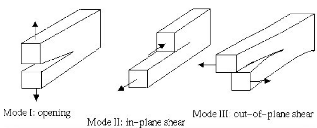
Fig. 4: The three modes of fracture. CPST occurs in Mode III fracture - PST occurs primarily in Mode II fracture.
