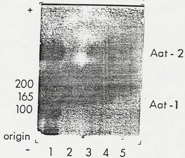
Photo 16 - Interspecific differences at the diagnostic Aat-1 locus. Each taxon has different electrophoretic alleles at this locus: Rainbow trout, Aat-1(100)-sample 1. Yellowstone cutthroat trout, Aat-1(165)-samples 2 and 3. Westslope cutthroat trout, Aat-1(200)-samples 4 and 5.
