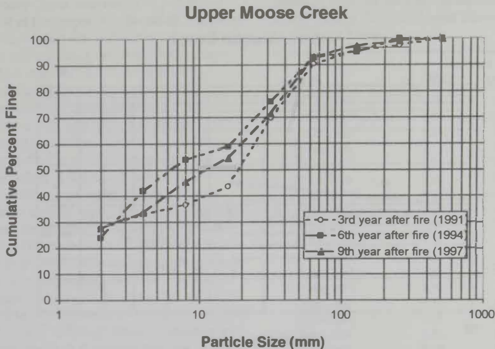
Figure 8. Cumulative particle size distributions, upper Moose Creek site.
