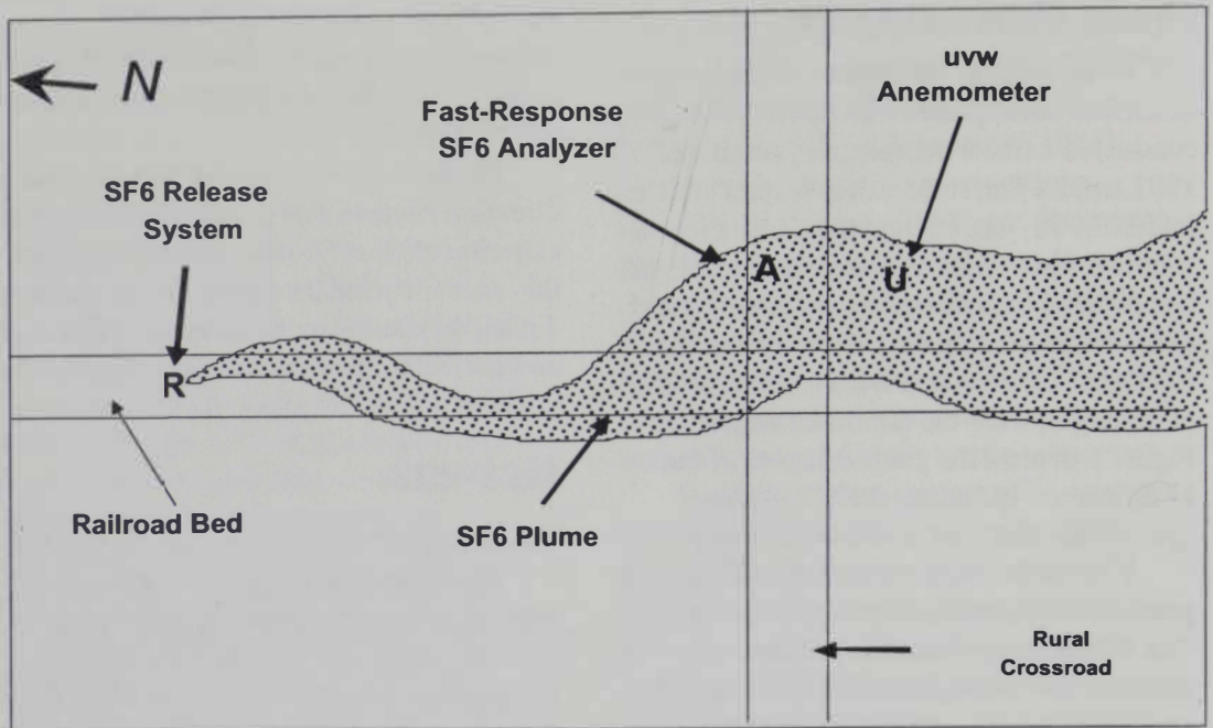
Figure 1. Example experimental setup during Galen tracer experiments.
