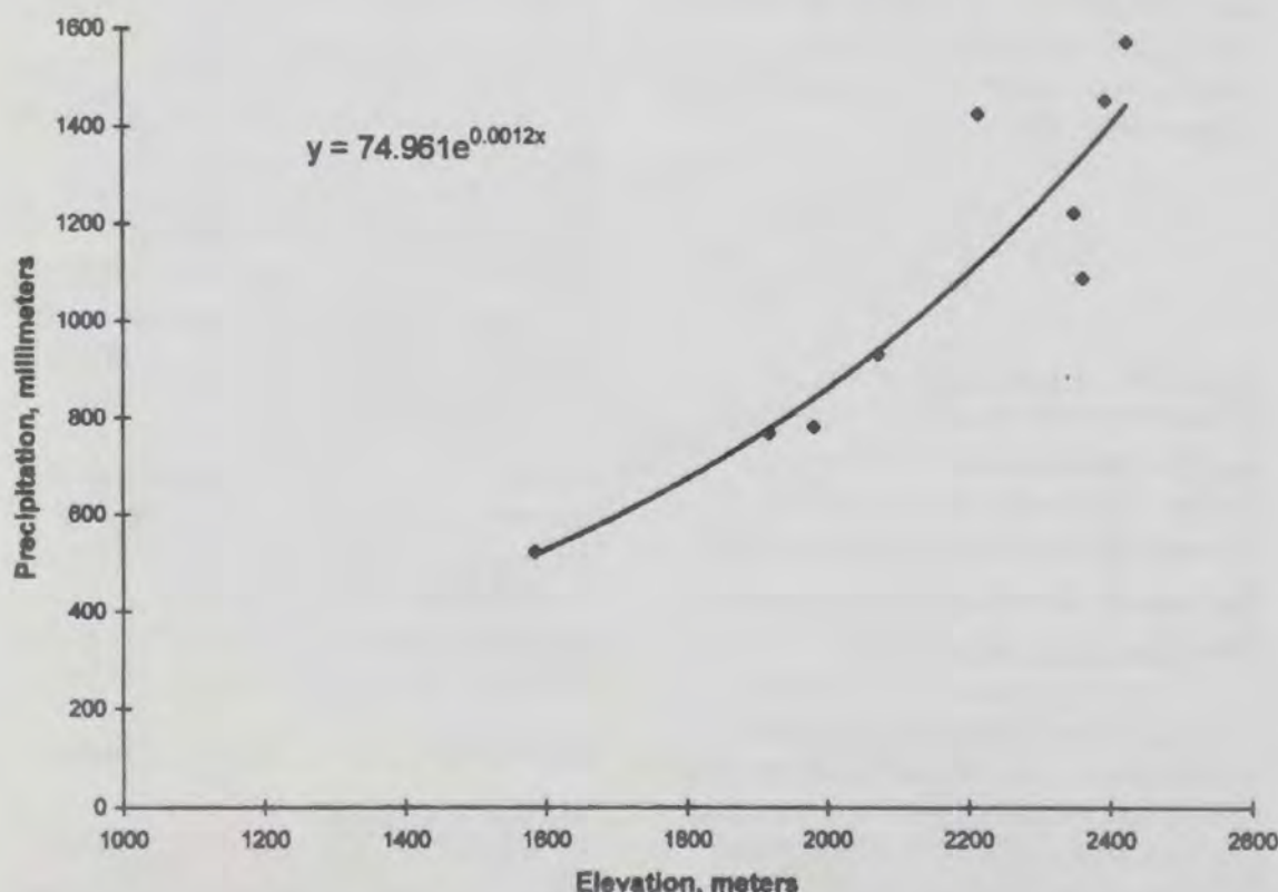
Figure 5. Mean annual precipitation as a function of altitude in western Yellowstone National Park and eastern Idaho.
