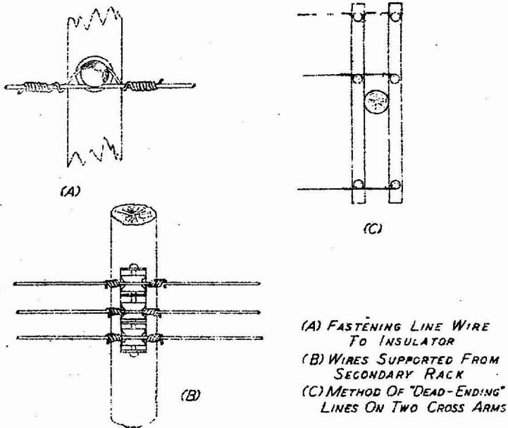
FIGURE 13. DETAILS OF TRANSMISSION LINE CONSTRUCTION
