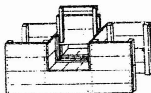
(E) WOOD HEAD GATE
