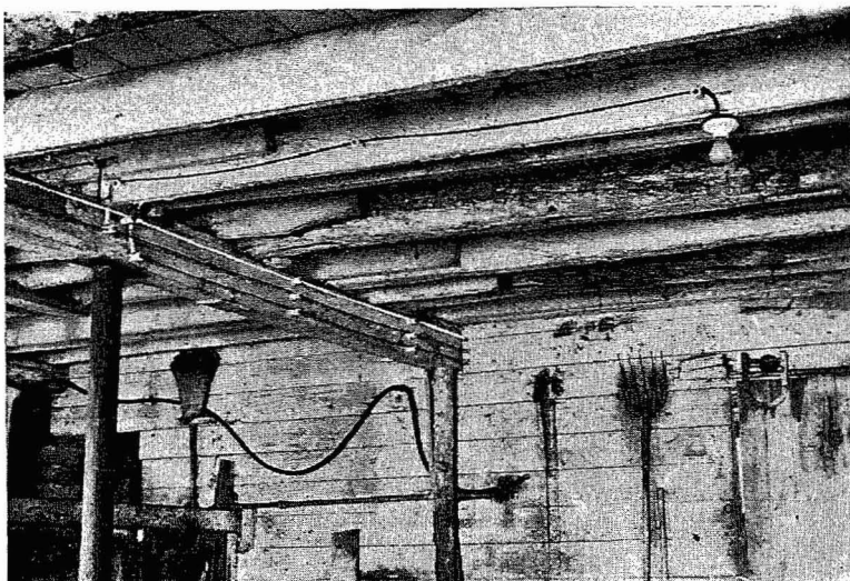
Figure 15. OPEN KNOB AND TUBE WIRING IN A BARN.
