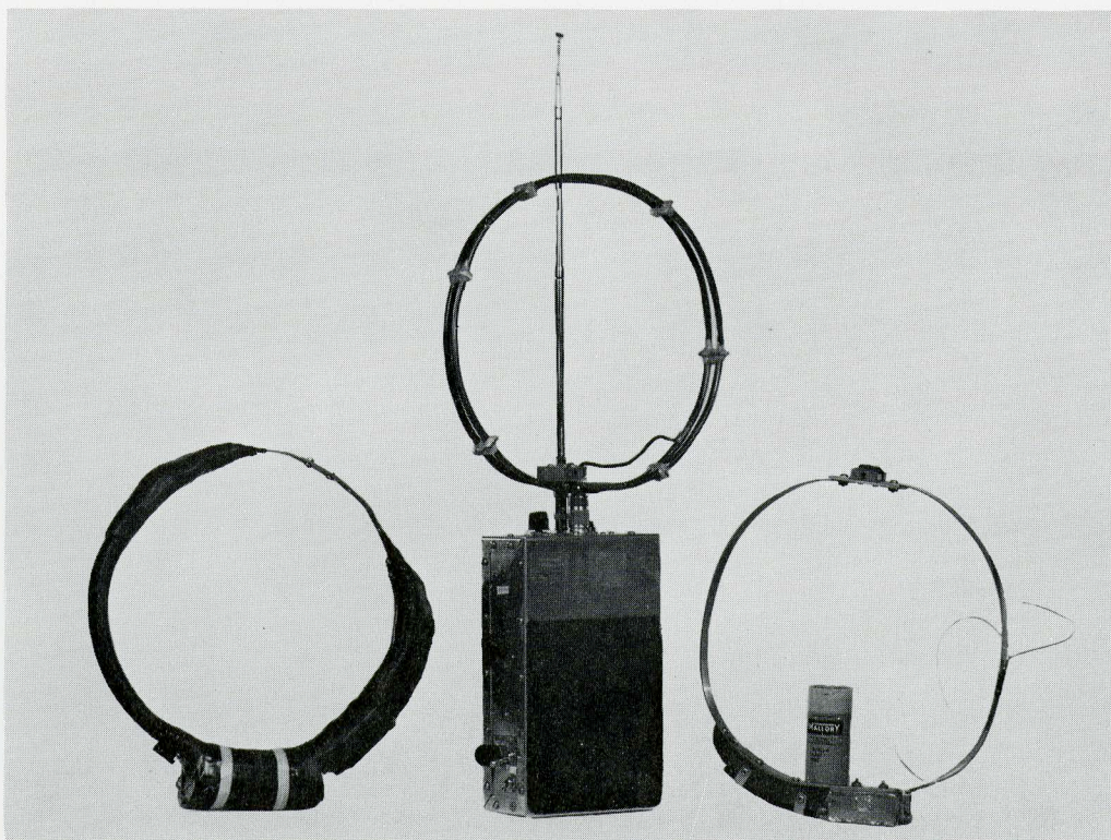
Fig. 3. Transmitter collars and a portable, directional receiver.
