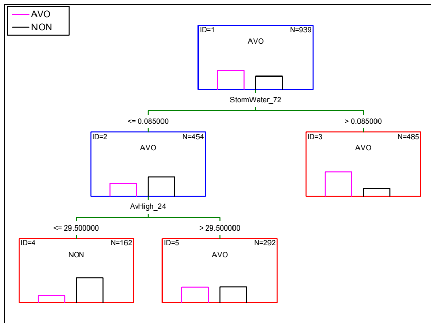
Figure 3: Avalanche day classification tree analysis following 10 fold cross validation showing Tree 8*. Tree 8* is calculated using a misclassification costs of two for false negatives and one for false positives, and has an overall accuracy of 68%, while avalanche days are much better predicted at 93%. Variable names used are as in Table 2.
