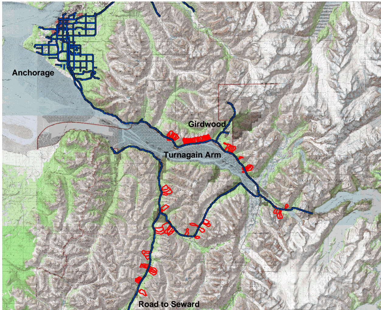
Figure 1: Location map showing the Seward highway (shown in blue), that connects Anchorage with Seward, Alaska, USA. The main avalanche paths are shown as the red polygons on the map. Key places of interest are labeled.
