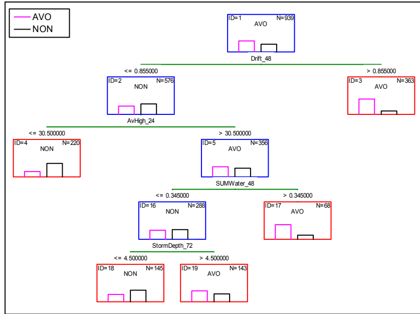
Figure 2: Avalanche day classification tree analysis following 10 fold cross validation showing Tree 8. Tree 8 is calculated using equal misclassification costs of one for any incorrect classification, and has an overall accuracy of 73%, while avalanche days are better predicted at 79%. Variable names used are as in Table 2.
