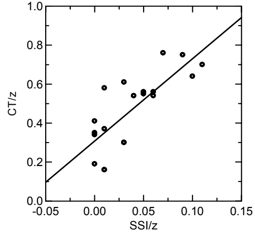
Figure 1: Compression Test results (CT/z) vs. Skier Stability Index (SSI/z). Both values were scaled to depth z . SSI was calculated for 11 manually observed flat field profiles taken during winter 2005-2006 in the surroundings of Davos. Only CT-results for layers of persistent grain types deeper than 15 cm from the snow surface were considered for regression ( N = 20 , p < 0.001 and R^2 = 0.61 ).
