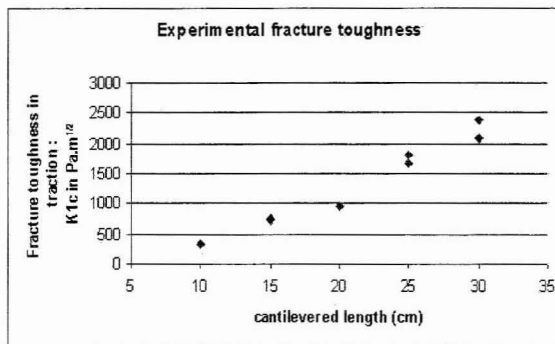
Figure 4: Measured tensile fracture toughnesses for different cantilevered lengths.
