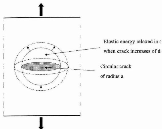
Figure 1: Stability of a circular crack under tensile loading.
