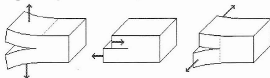
Figure 2: Different rupture modes: mode I or tensile (left), mode II and III or shear modes (center and right).
