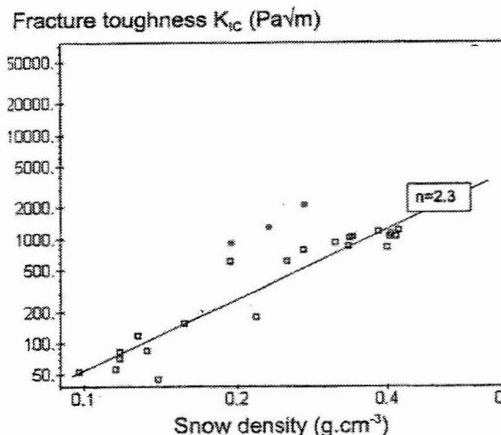
Figure 5: Measured tensile fracture toughnesses for different snow densities, compared with literature (open squares).
