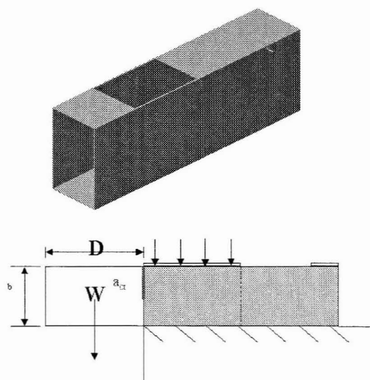
Figure 3: Experimental set-up for snow toughness measurements.
