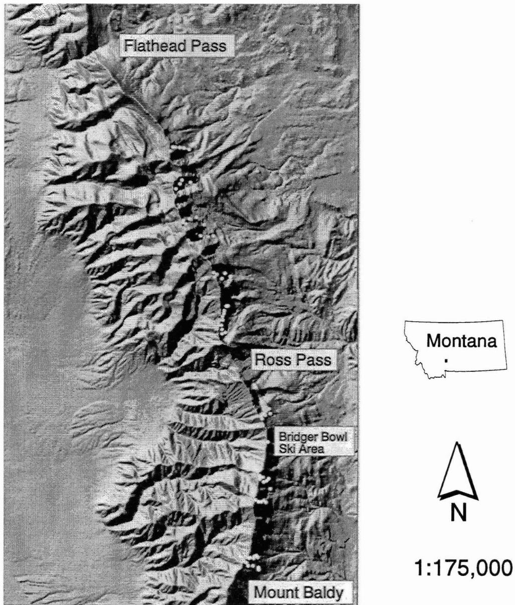
FIGURE 1: The Bridger Range is located approximately 5 km northeast of Bozeman, Montana, U.S.A. This hillshades map, generated with U.S. Geological Survey 30 m digital elevation models, shows the sampling locations (represented by the white dots) for this study. A helicopters shuttled teams to the ridgetop for sampling location access.
