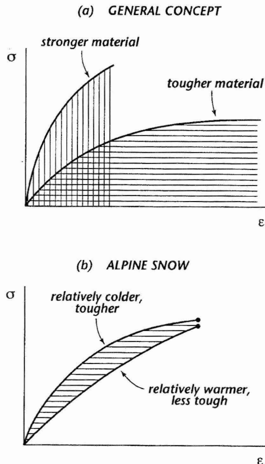
Figure 1:(a) Definitions of strength and toughness in terms of stress ( \sigma ) strain ( \epsilon ) curves. Strength is defined by the peak on the stress-strain curve. Toughness is defined as the area under the stress-strain curve until a peak is reached. Stiffness is defined as the initial slope of the stress-strain curve. (b) Schematic of stress-strain curves for alpine snow of two different temperatures: strength, toughness and stiffness decrease with increasing temperature.
