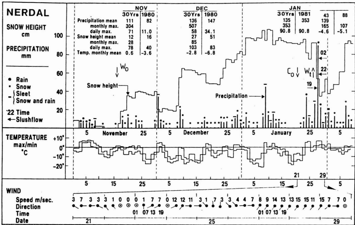
Fig. 13 The winter and current weather conditions leading to the catastrophic slushflows, in Sjäneshøia, Rana 27-28.01.1981. Weak cohesionless winter snowpack of coarse grains. Daily records from the DNMI observation station 7940 Nerdal, 2.5 km away.
