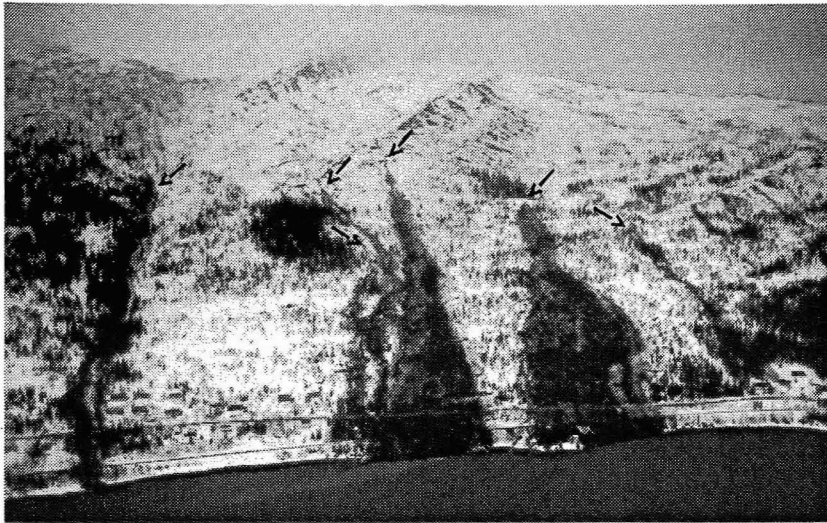
Fig. 9 The slushflows on this sparsely forested hillside in Sjønesheia, Rana, 27-28.01.1981, closed the road and the railway between South and North Norway for 2 and 4 days, respectively. The arrows indicate the starting zones of six slushflows. (Photo O.I. Tysnes, Dagbladet)
