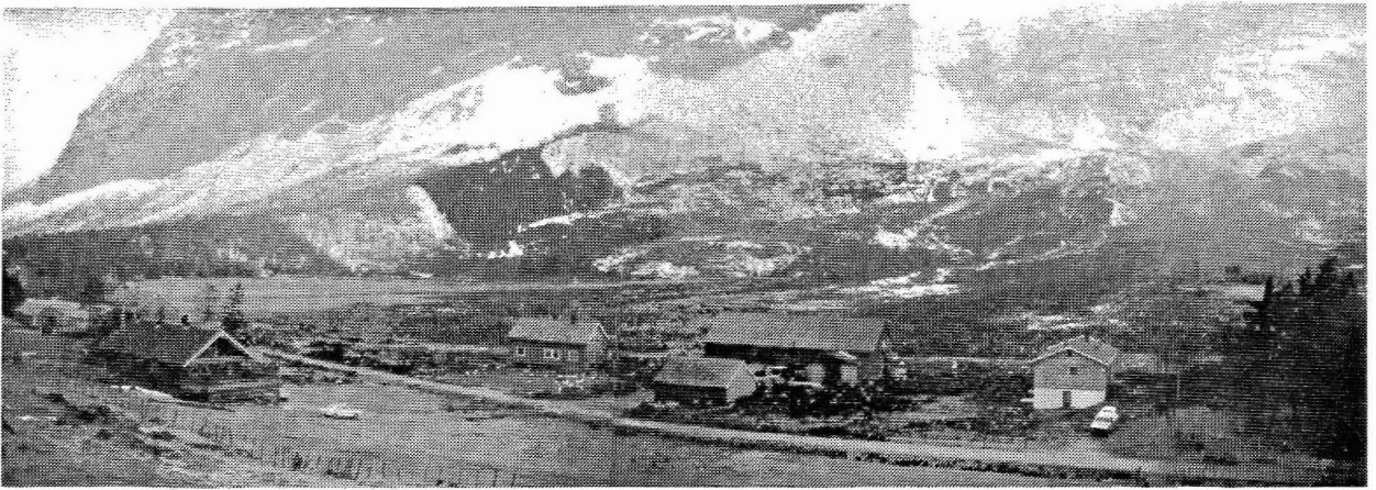
Fig. 1 A huge slushflow released from a low-grade snowfield of high water content on the mountain slope has destroyed the farm buildings at Fivelstad, Stranda 05.02.1990 (Photo K. Kristensen, NGI)
