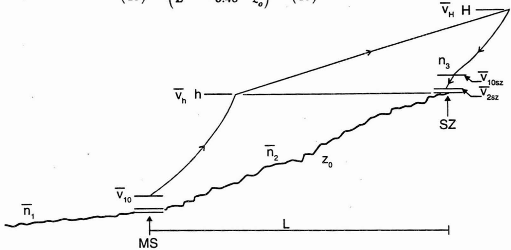
Fig. 17. Principle of transformation of recorded wind speed at meteorological station to starting zone.
