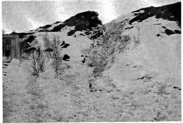
Fig. 3 The slushflow in Hammerfest was released in a drainage channel due to rain and snow-melt 15.02.1994. (Photo K. Lied, NGI)
