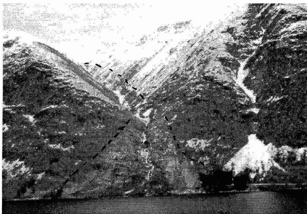
Fig. 6 A destructive flood wave was created in Vete-fjorden by the impact of a huge slushflow 28.04.1994. The slushflow was 600 meters wide by the fjord. (Photo E. Hestnes, NGI)
